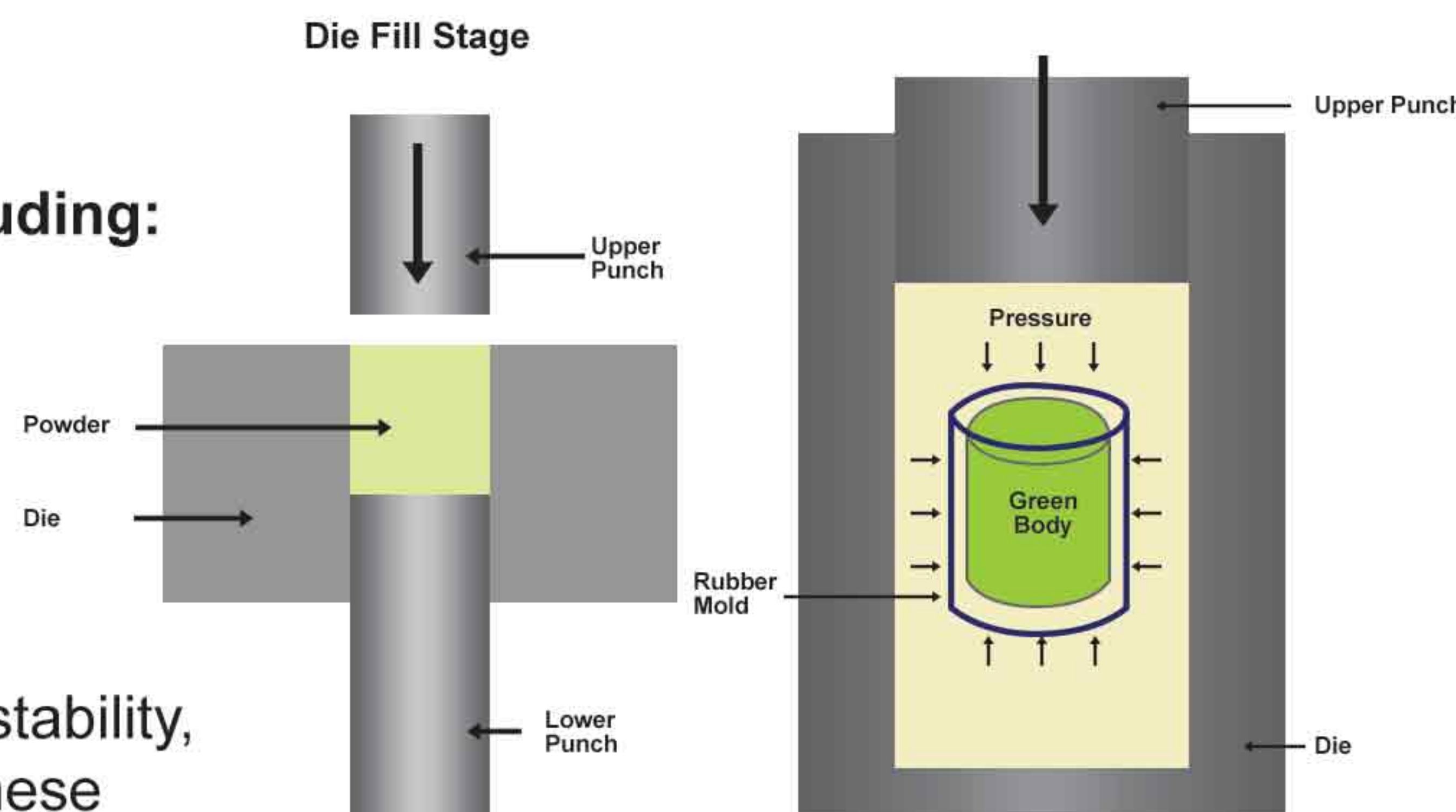
Cold Isostatic Pressing
